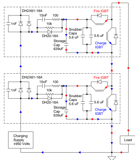
Figure 3: Marx double-cell circuit schematics.
