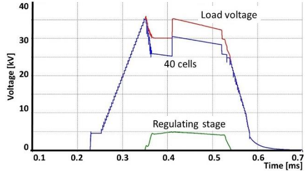
Figure 2: Modulator voltage waveform simulation.
