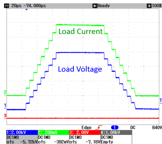
Figure 5: Waveforms for 9 Marx switching cells. Ch. 2: load current (100A/V) and Ch. 1: load voltage
