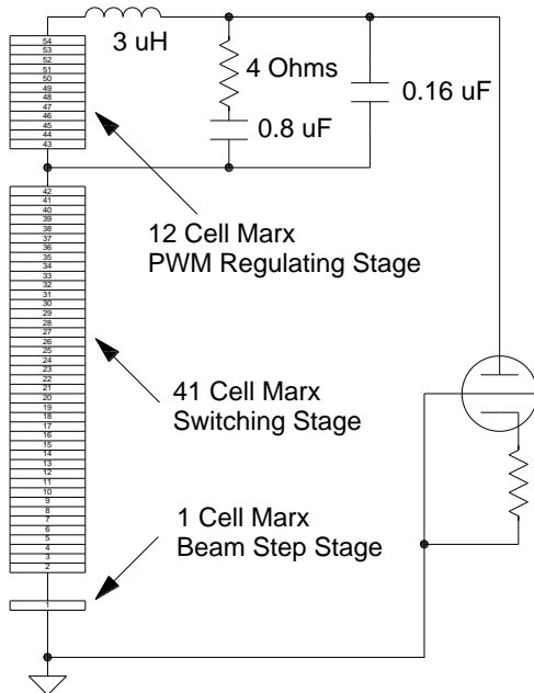
Figure 1: Full Marx modulator block diagram.
