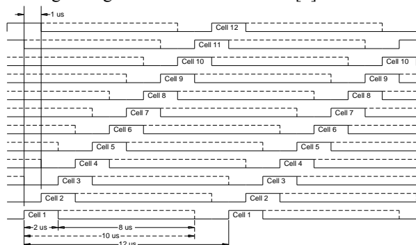
Figure 4: Regulating cells PWM waveforms.
